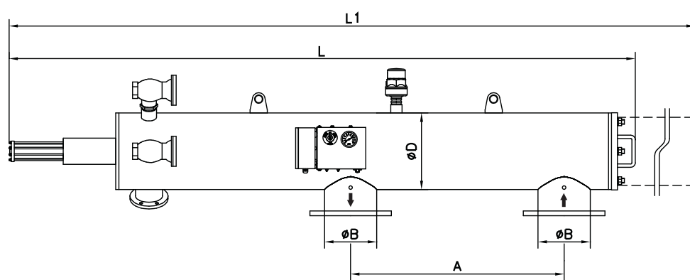
Parallel Inlet/Outlet Model (PS, PE)
